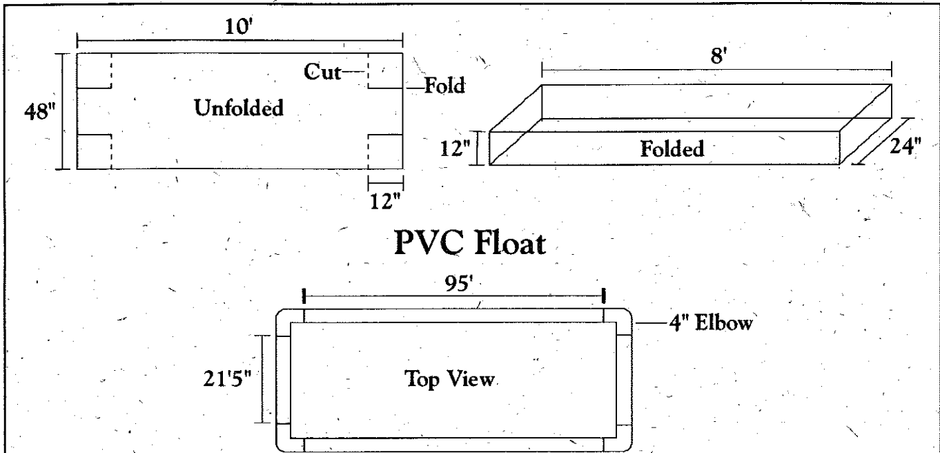
Figure 2. Taylor float design and approximate materials cost.
